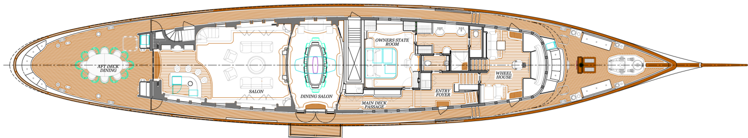
MAIN DECK
