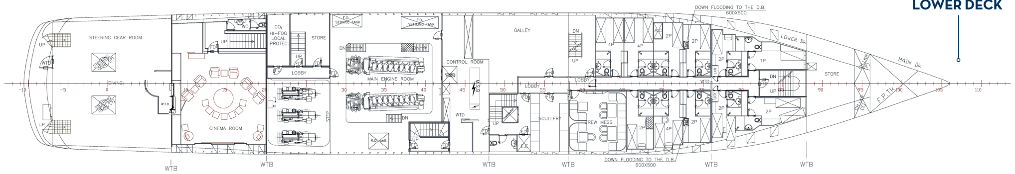
LOWER DECK
