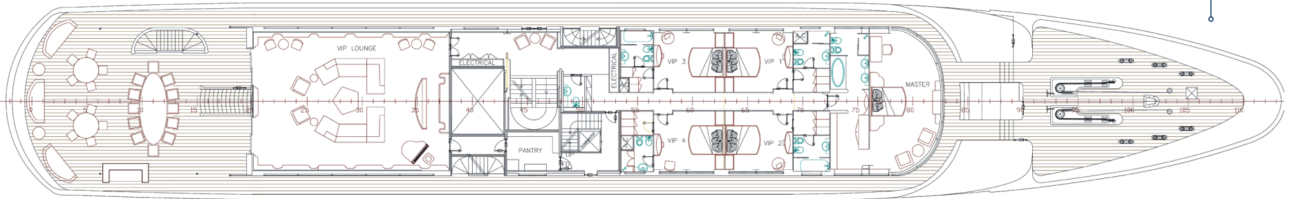
MAIN DECK
