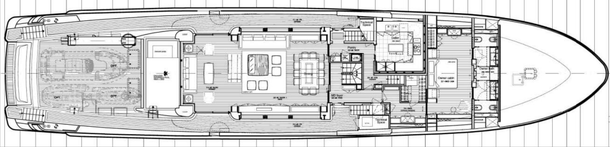
MAIN DECK
